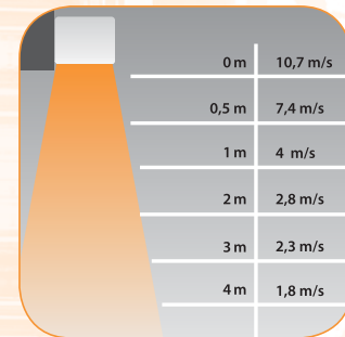
Distance/air speed
