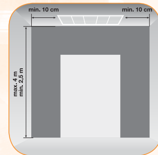
Fitting height
